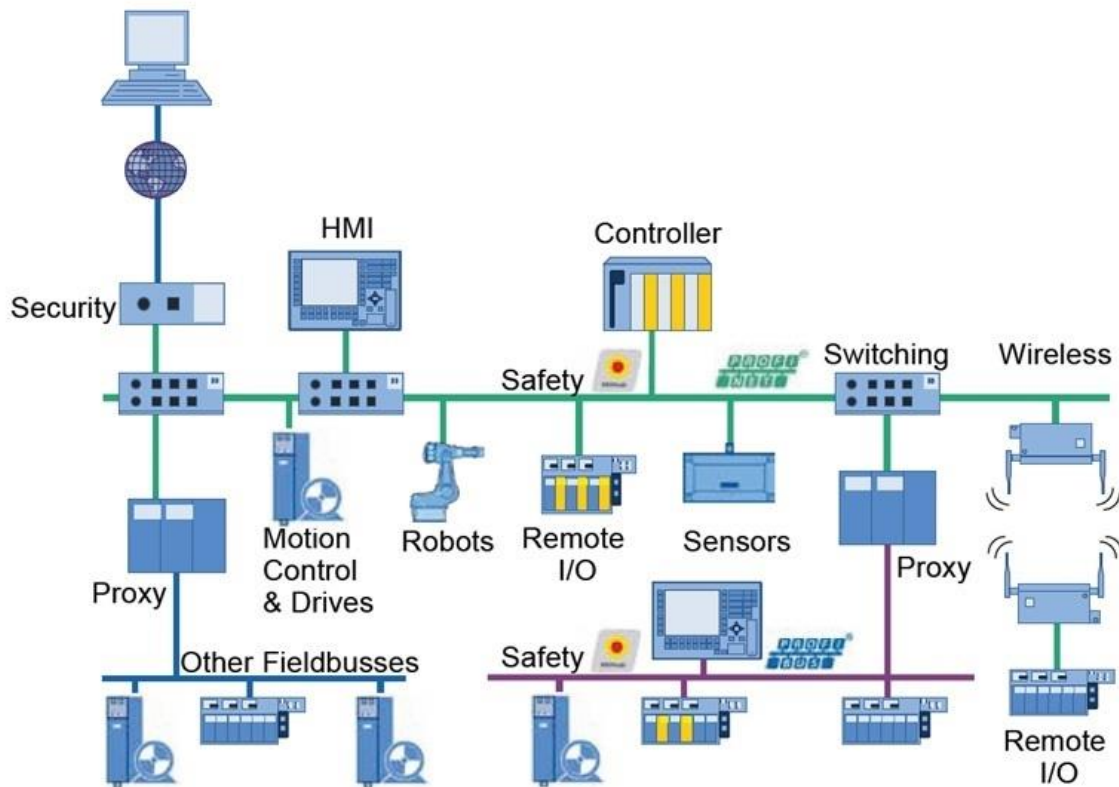
Figure 3: A Profinet network in an automation system (Source: Profibus International)
